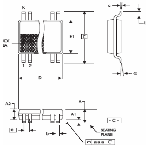
56 PIN TSSOP-240mil
